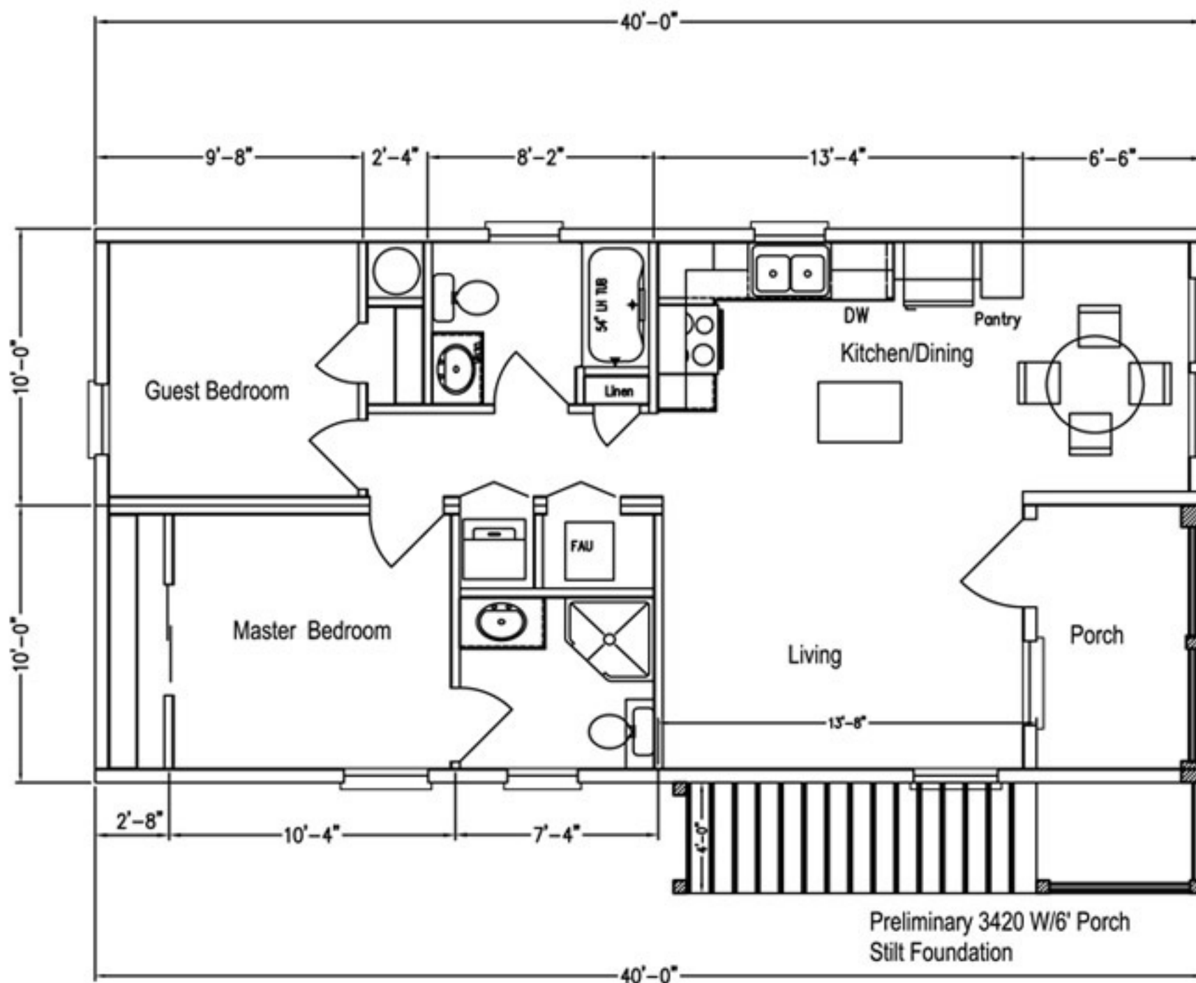
Preliminary 3420 W/6' Porch Stilt Foundation
