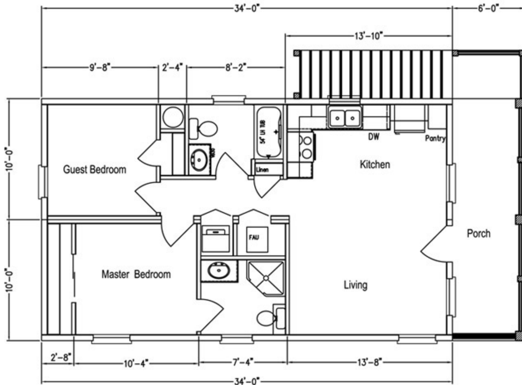
Preliminary 3420 W/6' Porch Stilt Foundation
